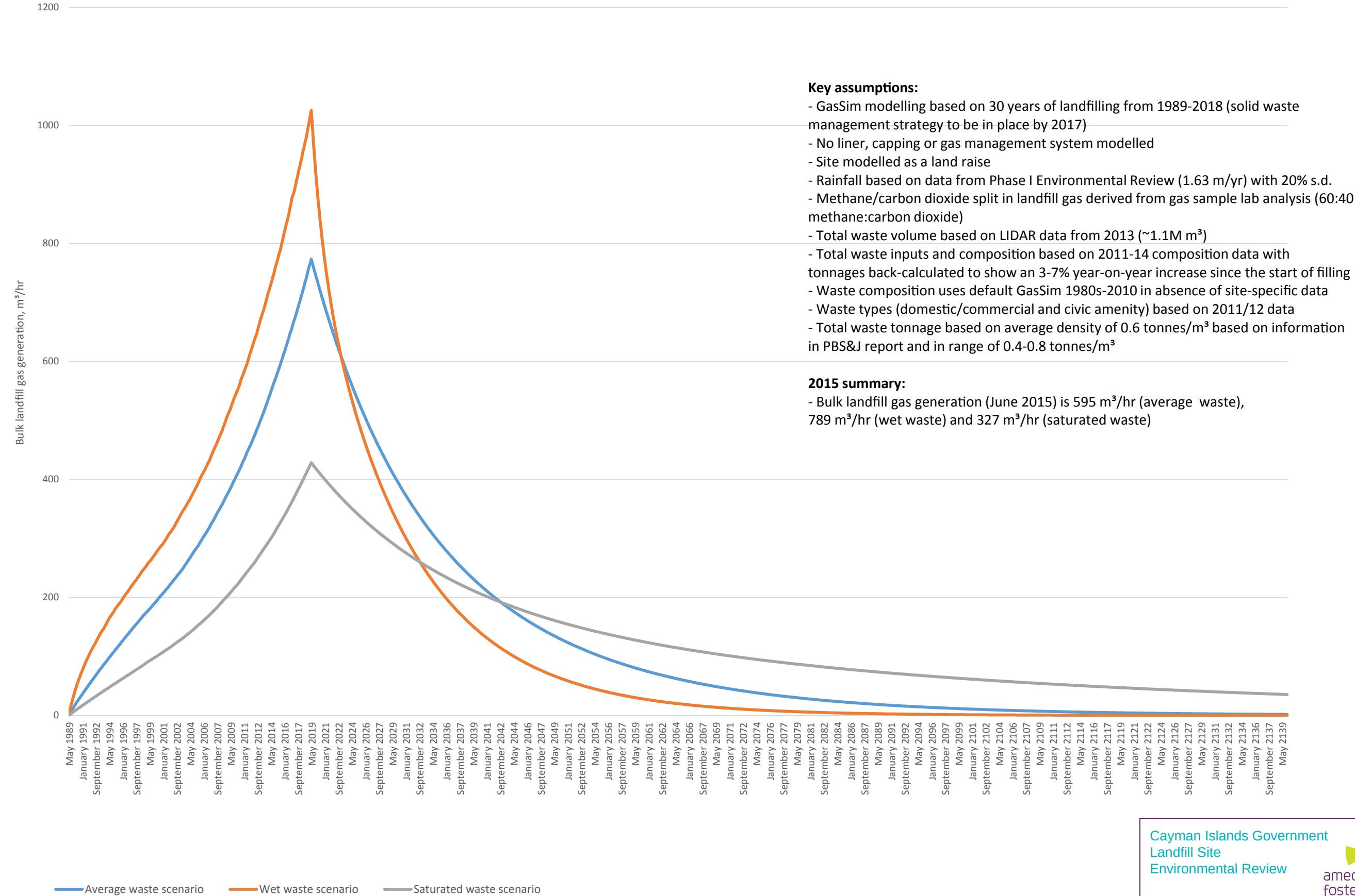
Bulk landfill gas generation at George Town landfill site from GasSim modelling
